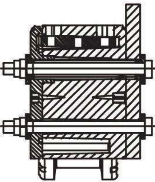
Side connection
