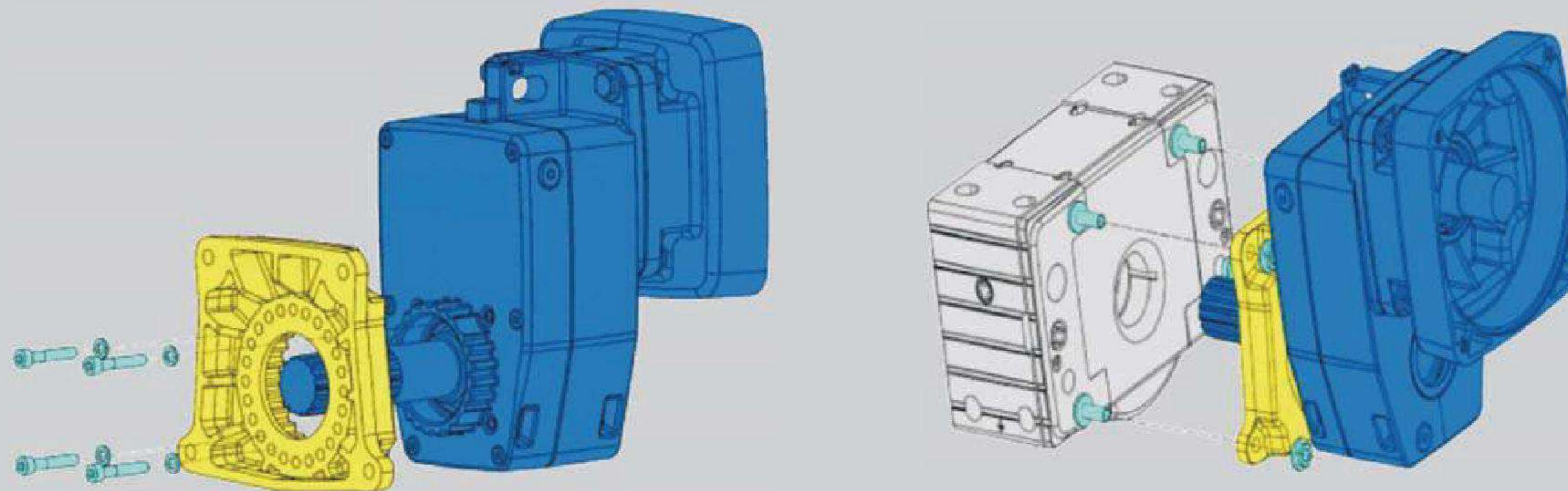
DRS112-DRS200 Connection the flanges with the motor
