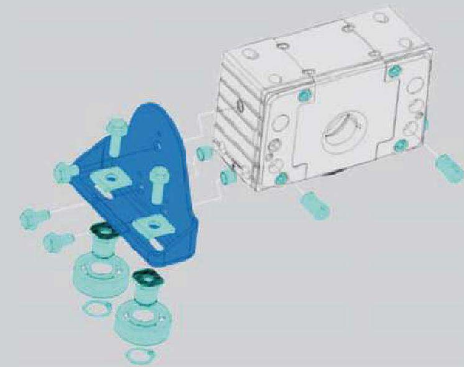
DRS112-DRS200 Use the guide wheel
