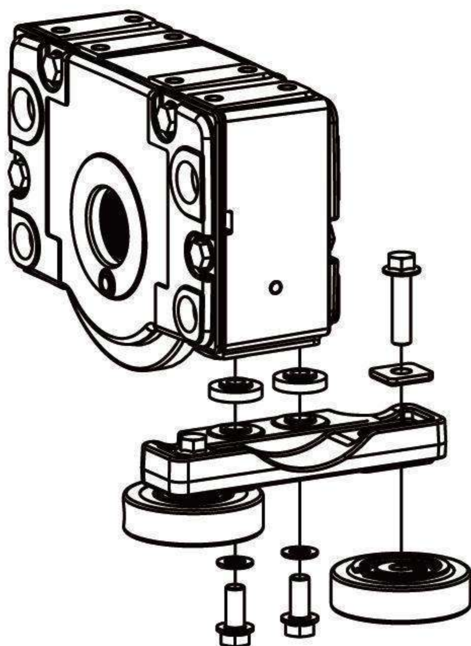
DRS250-500 Horizontal guide rollers
