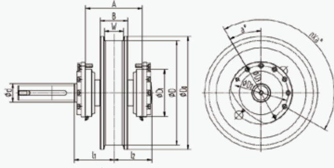
Φ500-710 Active Wheel Set
