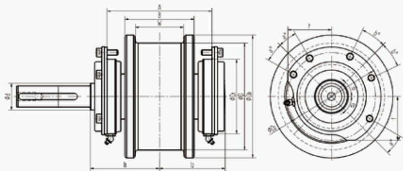
Φ200-400 Active Wheel Set
