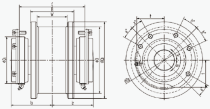
Φ200-400 Idle Wheel Set
