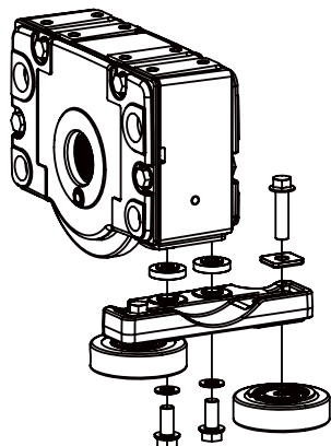
DRS250-500 Horizontal guide rollers
