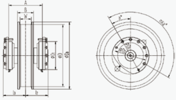
Φ500-710 Idle Wheel Set
